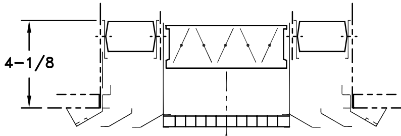
DIFFUSER WITH OPTIONAL O.B. SUPPLY AND O.B. RETURN DAMPER
