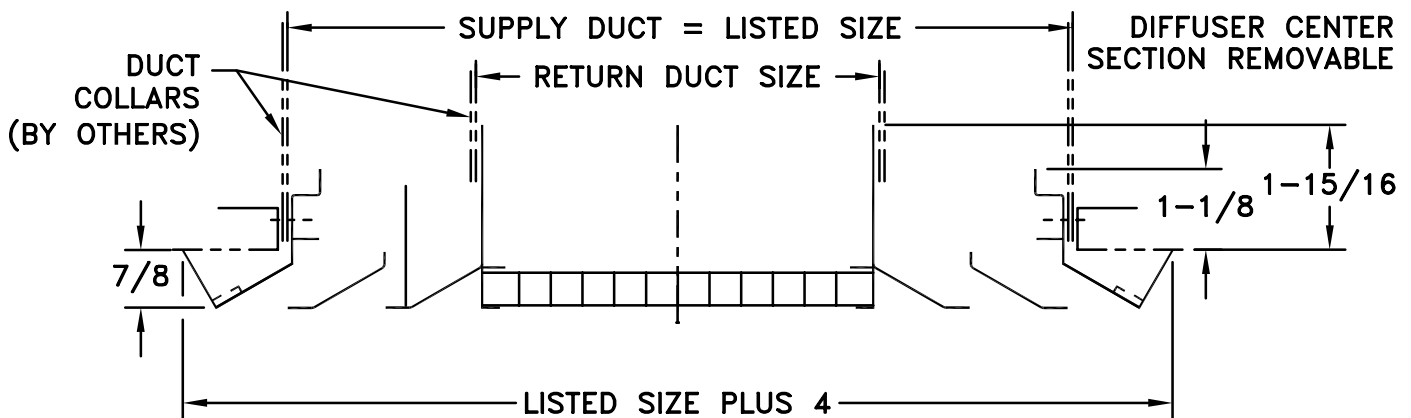
DETAIL OF OPTIONAL LEAF SUPPLY DAMPER WHEN RETURN DUCT SIZE IS 3 INCHES LESS THAN SUPPLY DUCT SIZE
